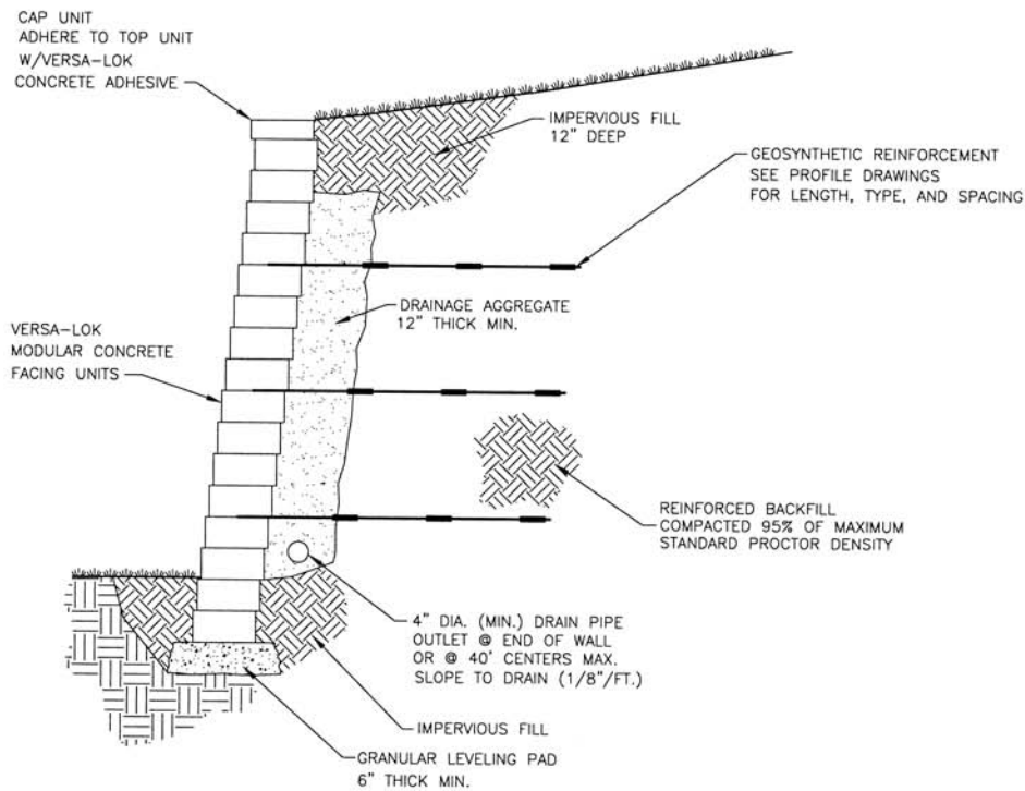
TYPICAL SECTION—REINFORCED RETAINING WALL
