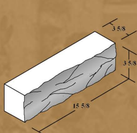
4" x 4" x 16"
