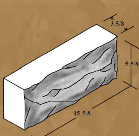
4" x 6" x 16"
